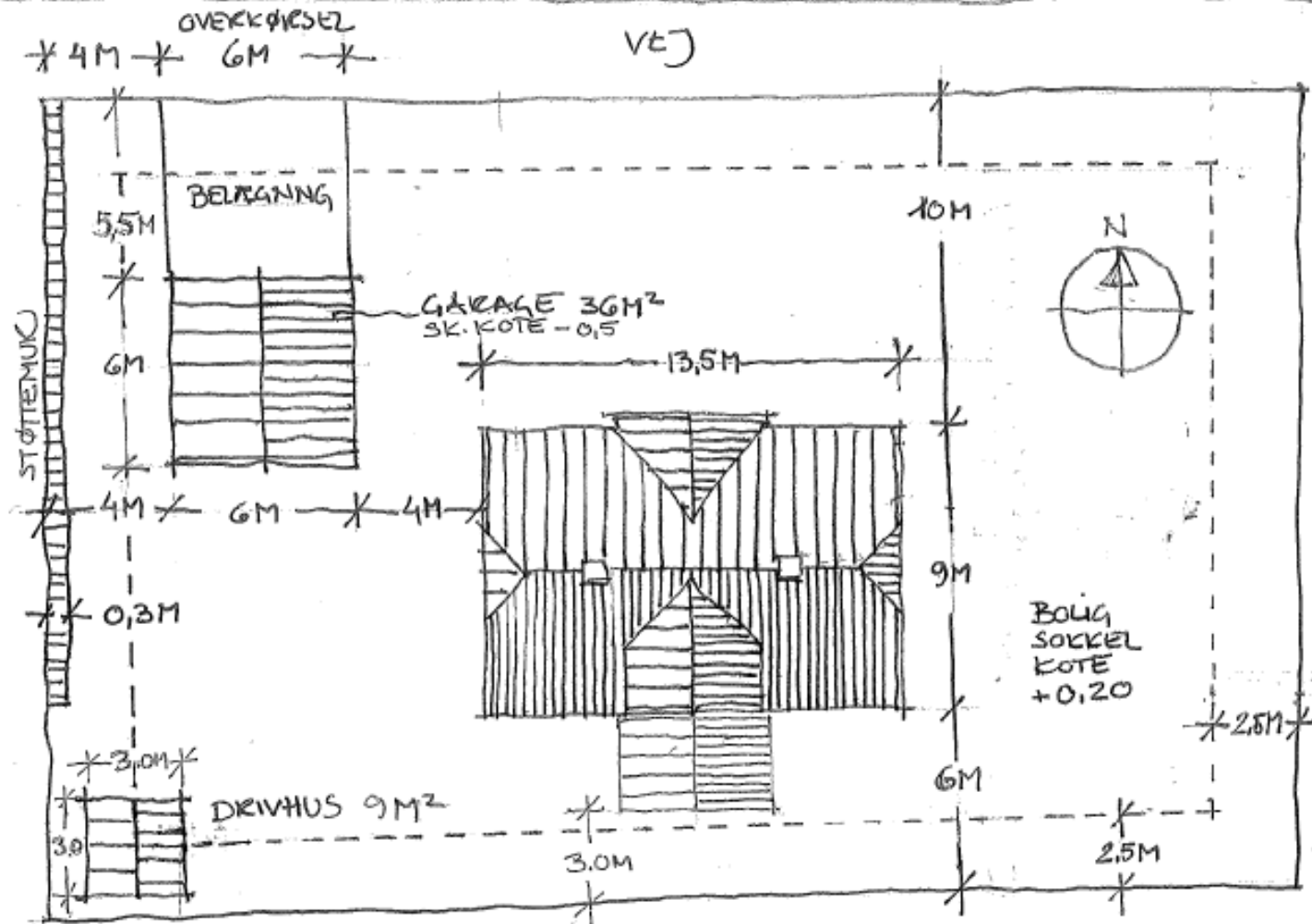
SITUATIONSPAN 1:200
